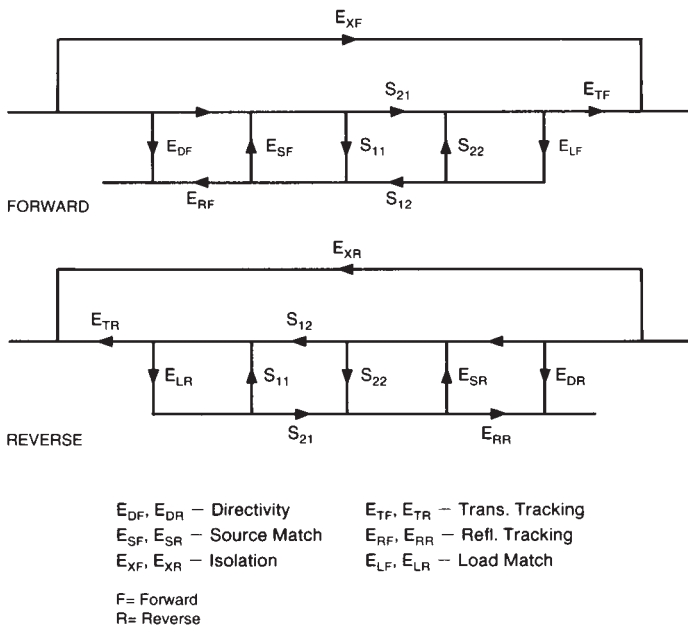
Figure 3. Two-port 12-term error model.
