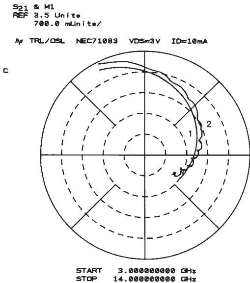
Figure 16. Example measurement of a linear FET on the microstrip PC board compared to measurement in a de-embedded test fixture (Keysight 85041A). (1) de-embedded measurement (2) TRL calibration using PC board standards.
