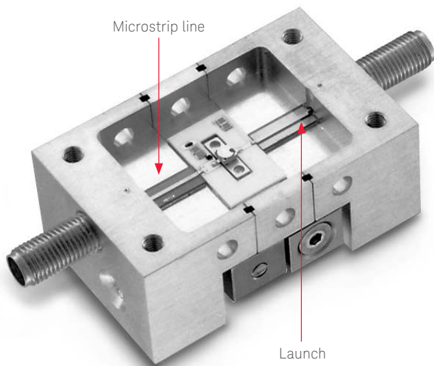
Figure 1. Microstrip test fixture.
