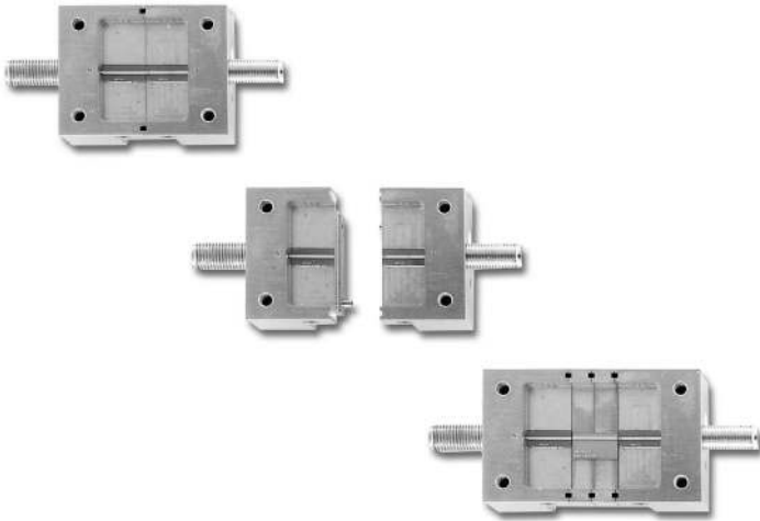
Figure 10. Calibration steps for a microstrip test fixture.
