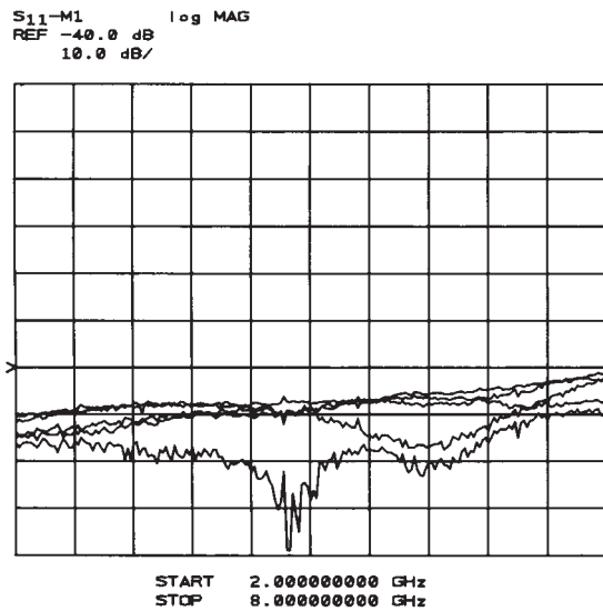
Figure 19. Connection repeatability of the microstrip test fixture.
