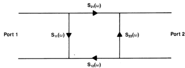
Figure 2. S-Parameter Flowgraph Notation.
