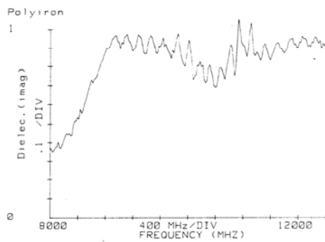
e. \epsilon''_r for Polyiron
