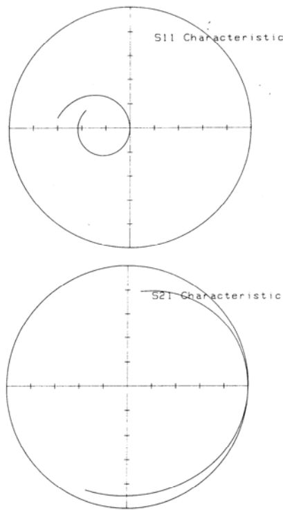
B. In Waveguide Sample Holder (Full Scale = 1)
