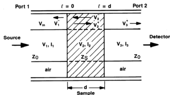
Figure 1. Air Line with Filled Material.
