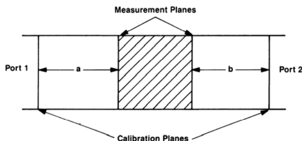
Figure A2. Reference Plane Rotation
