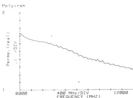
d. \mu'_r for Polyiron
