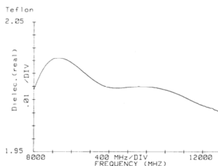
B. With Time Domain Gating (gate width 2 ns).
