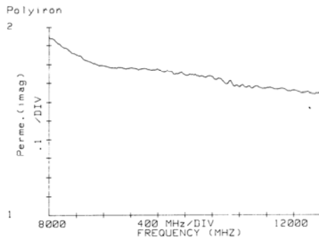
f. \mu''_r for Polyiron
