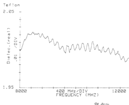
A. No Time Domain Gating.
