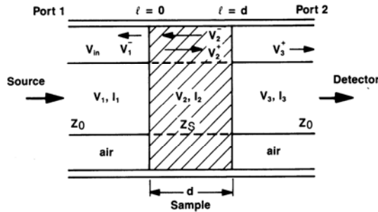
Figure A1. Air Line with Filled Material
