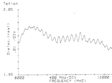
a. \epsilon'_r for Teflon
