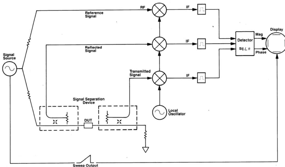
Figure 3. Network Analyzer Simplified Block Diagram.
