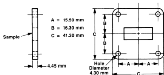
Figure 4. Coaxial and Waveguide Sample Holders.
