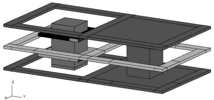
Fig. 7. Single via structure. Two ports are defined between vertical conductor and top (bottom) ground planes.
