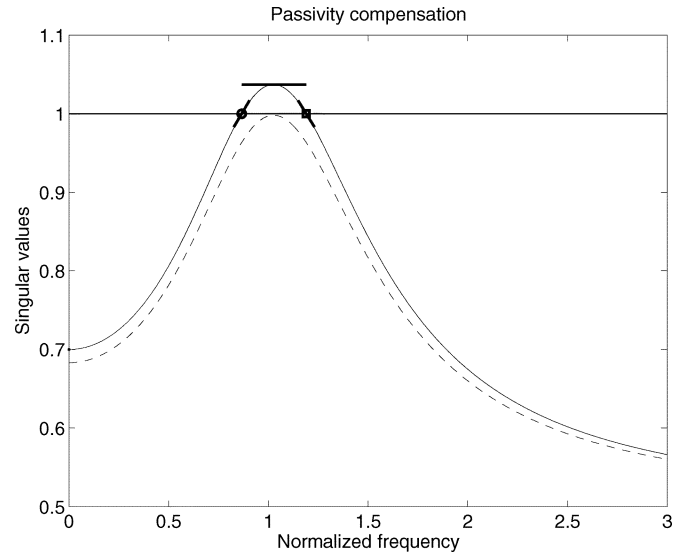
Fig. 6. Singular value plot (solid line) for the test system (69) and for the compensated system obtained using \alpha = 0.3 (dashed line). Only one iteration is required for the passivity compensation.
