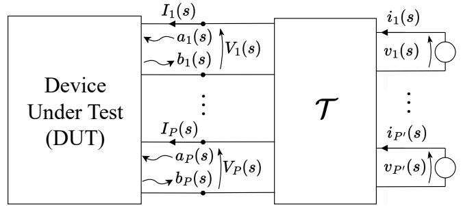
Fig. 1. A P -port representing the structure under modeling inserted in a larger electrical network. The device to be modeled (DUT) is loaded with a generic termination network \mathcal{T} . Hollow circles represent either ideal current or voltage sources.
